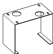
Anchor bracket
