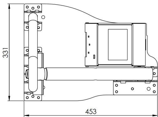
Barrier Raised - Top View
